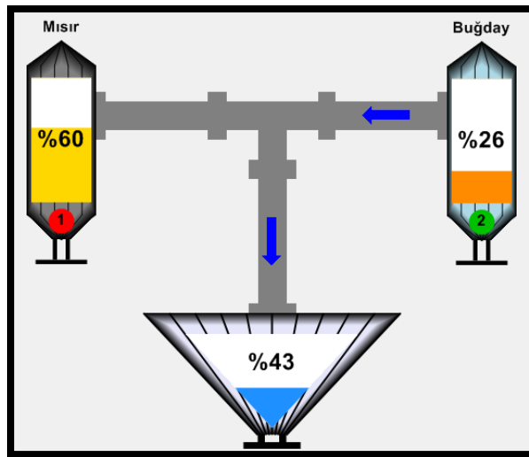
Silo, Mixture Tank and Pipe Components
